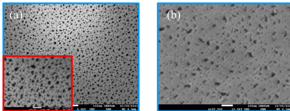
Top view of porous silicon membrane before (a) and after (b) ALD material coating.
